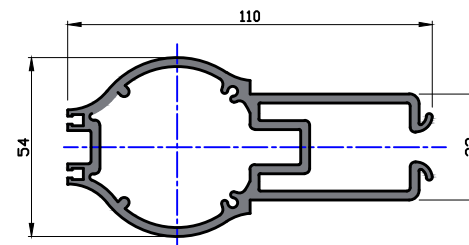
Part No. 404-101
