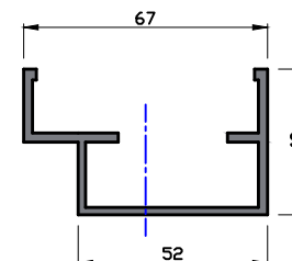
Part No. 515-151
