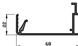
Part No. 606-155
