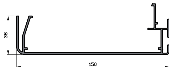
Part No. 606-152
