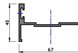
Part No. 515-152
