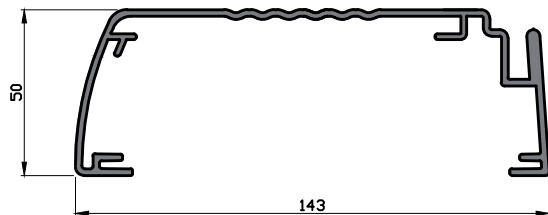
Part No. 505-110
