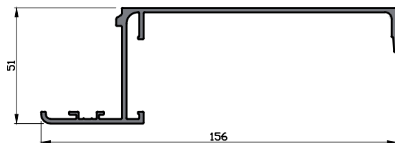
Part No. 606-151
