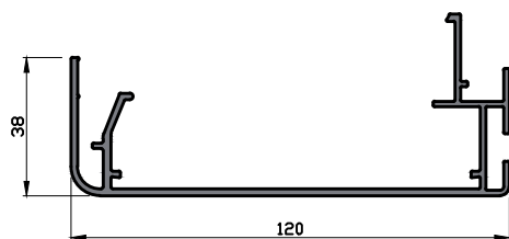
Part No. 606-153
