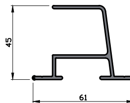
Part No. 606-159
