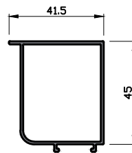
Part No. 606-158
