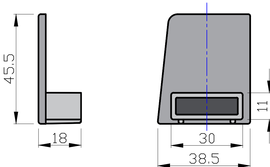
Part No. 606-123 LHS
