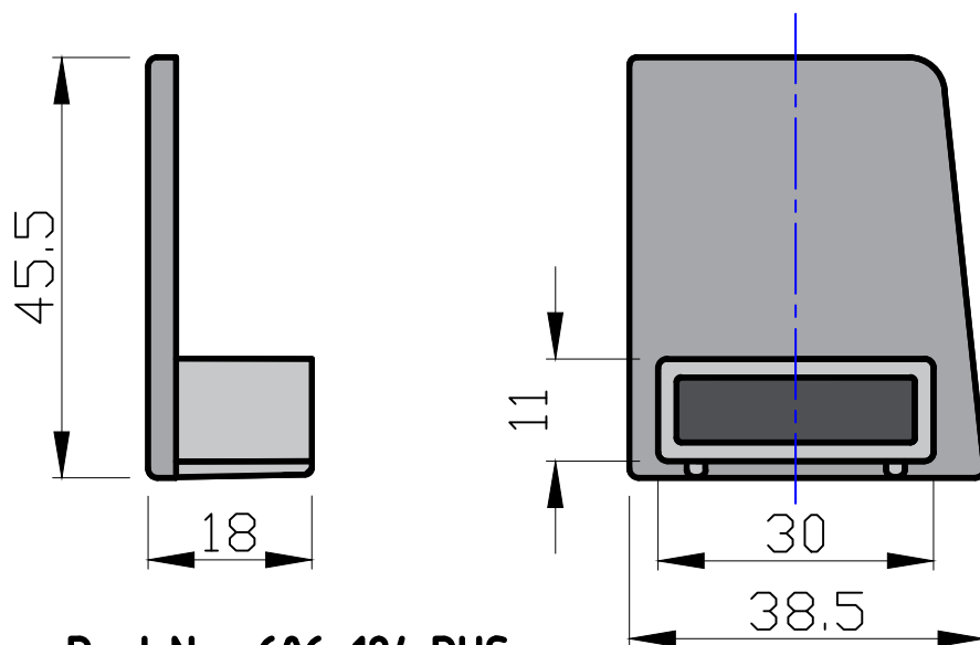
Part No. 606-124 RHS
